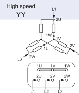
Centrifugal drive, Dahlander connection
