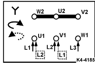
Star connection
